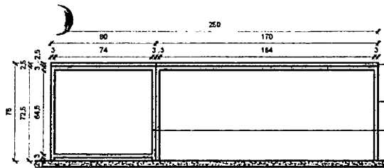
2 VISTA FRONTAL - MESA BANANA 1:20
